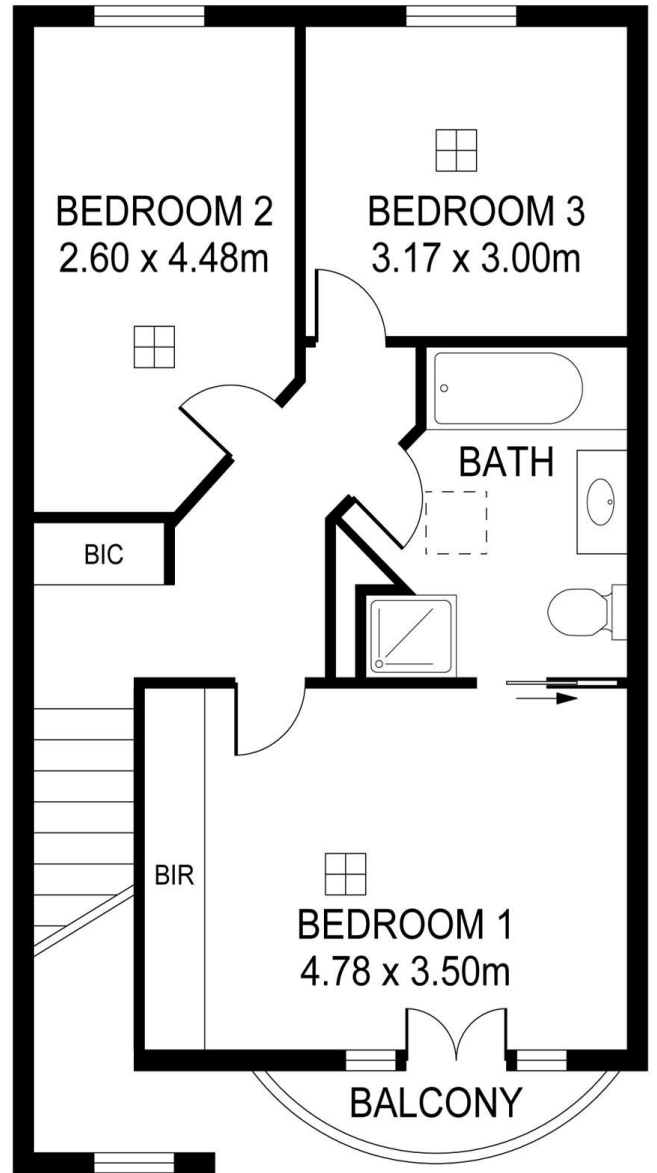
FIRST FLOOR - 58 SQM
